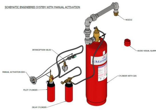
SCHEMATIC ENGINEERED SYSTEM WITH MANUAL-ELECTRIC ACTIVATION
