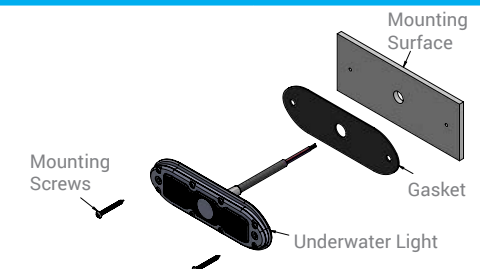
SCM-AL-MINI-TRACK-1M
