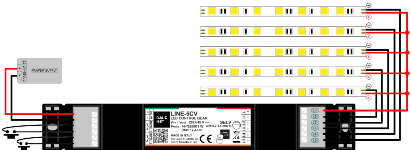
Figure 2: Connection diagram for White or Single-Color LED loads
