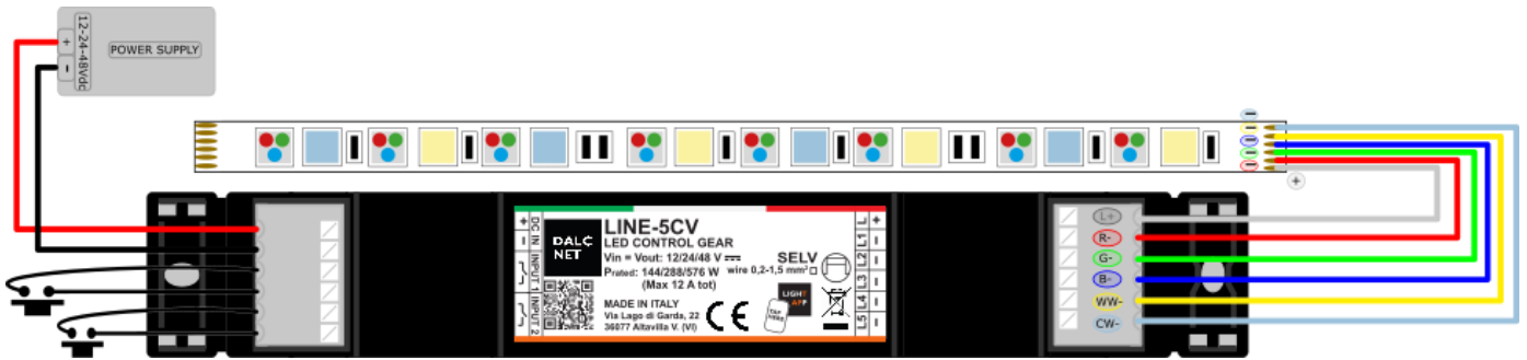
Figure 6: Connection diagram for RGB+TW LED load
