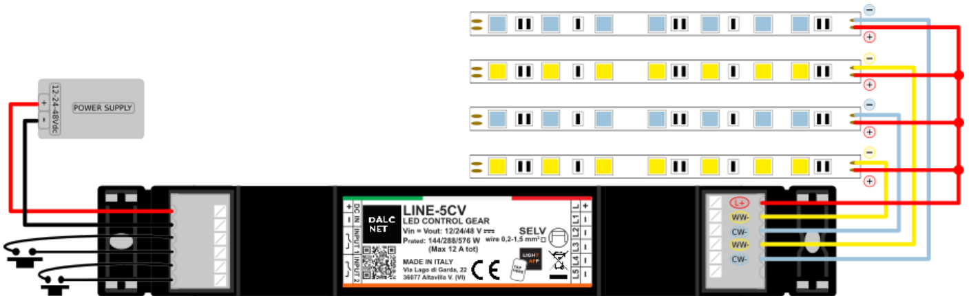
Figure 3: Connection diagram for Tunable White LED loads
