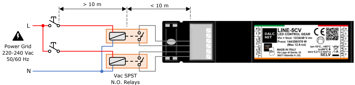
Figure 8: Local Command connection diagram for Long Distances
